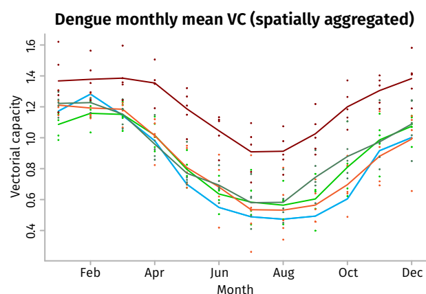
FIGURE 7: Monthly mean vectorial capacity (VC) in Vanuatu for dengue fever. Modelled estimates for 2015 (baseline) are presented together with 2035 and 2085 estimates under low emissions (RCP2.6) and high emissions (RCP8.5) scenarios
