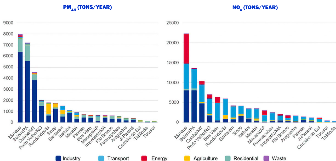
FIGURE 5. DISTRIBUTION OF EMISSION SOURCES BY AMAZONIAN CITY.
